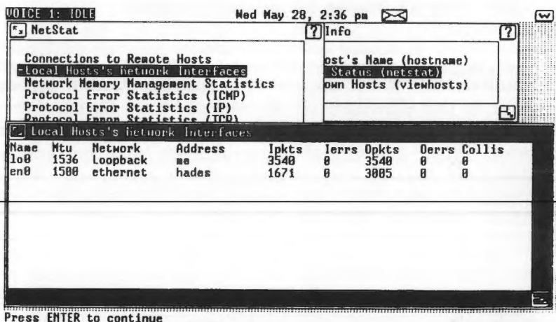
Figure 6-34. Local Host's Network Interfaces
