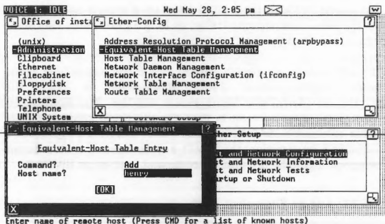
Figure 6-7. Adding an Entry to the Equivalent-Host Table
