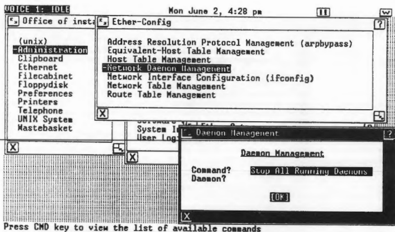
Figure 6-20. Stopping All Running Daemons
