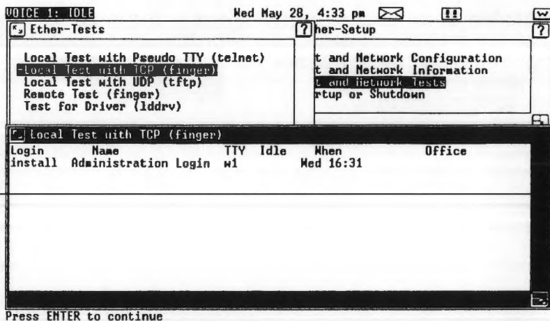
Figure 6-45. Testing with TCP
