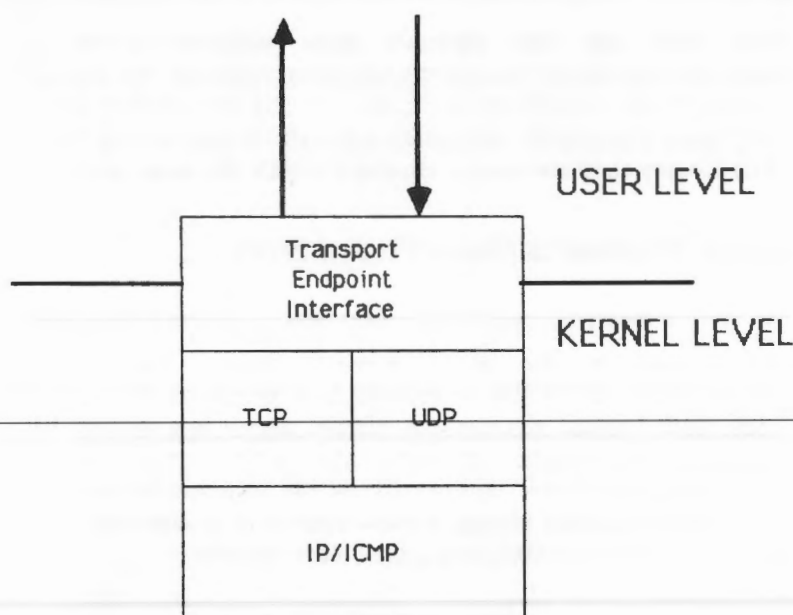
Figure 2-2. Network Pseudo Driver Structure
