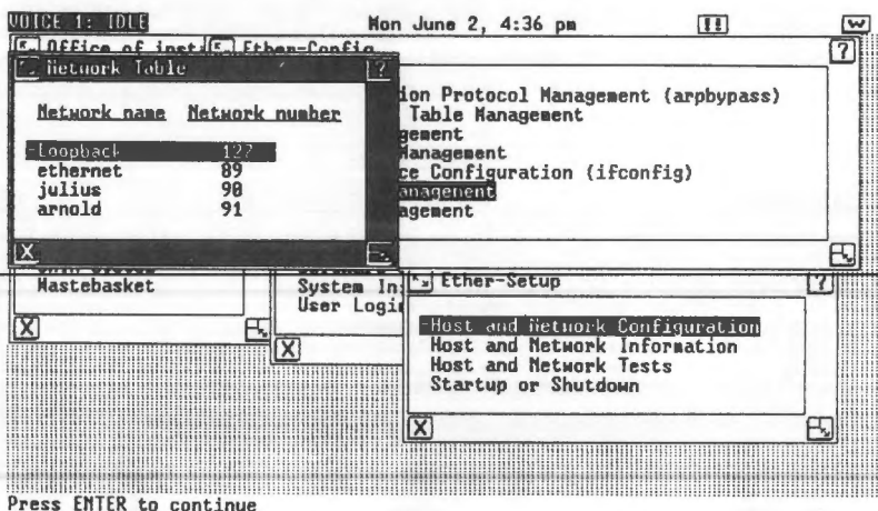
Figure 6-26. Showing the Network Table
