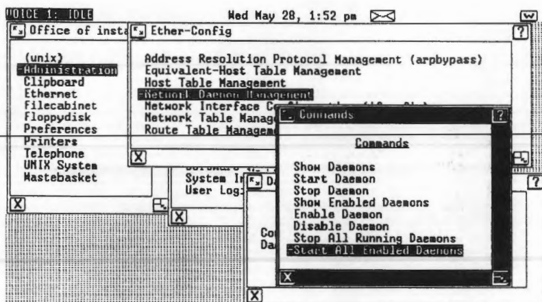
Figure 6-13. Network Daemon Management Commands
