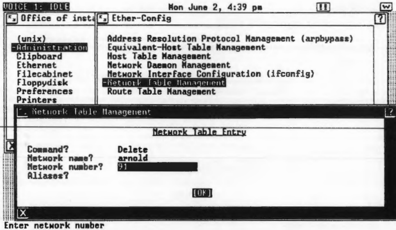
Figure 6-25. Deleting a Network Table Entry
