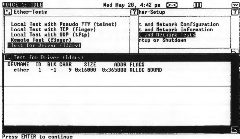
Figure 6-44. Testing the Network Driver
