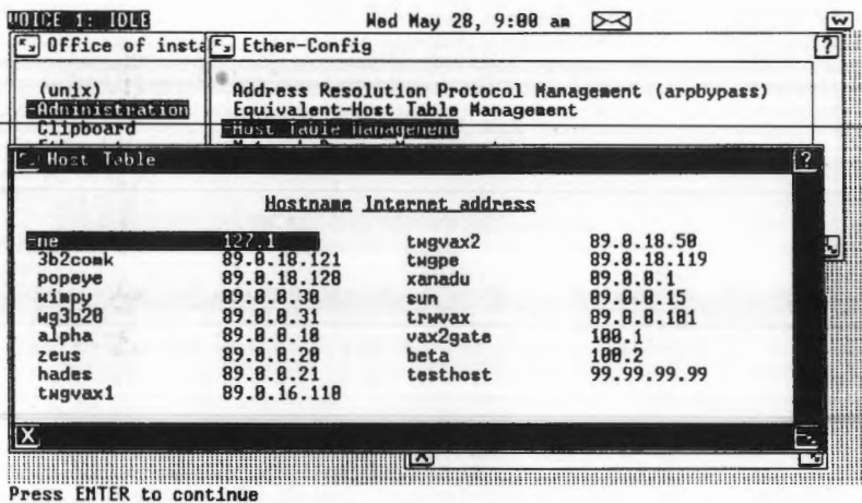
Figure 6-12. Showing the Host Table
