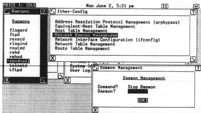
Figure 6-16. Stopping the sendmail Daemon
