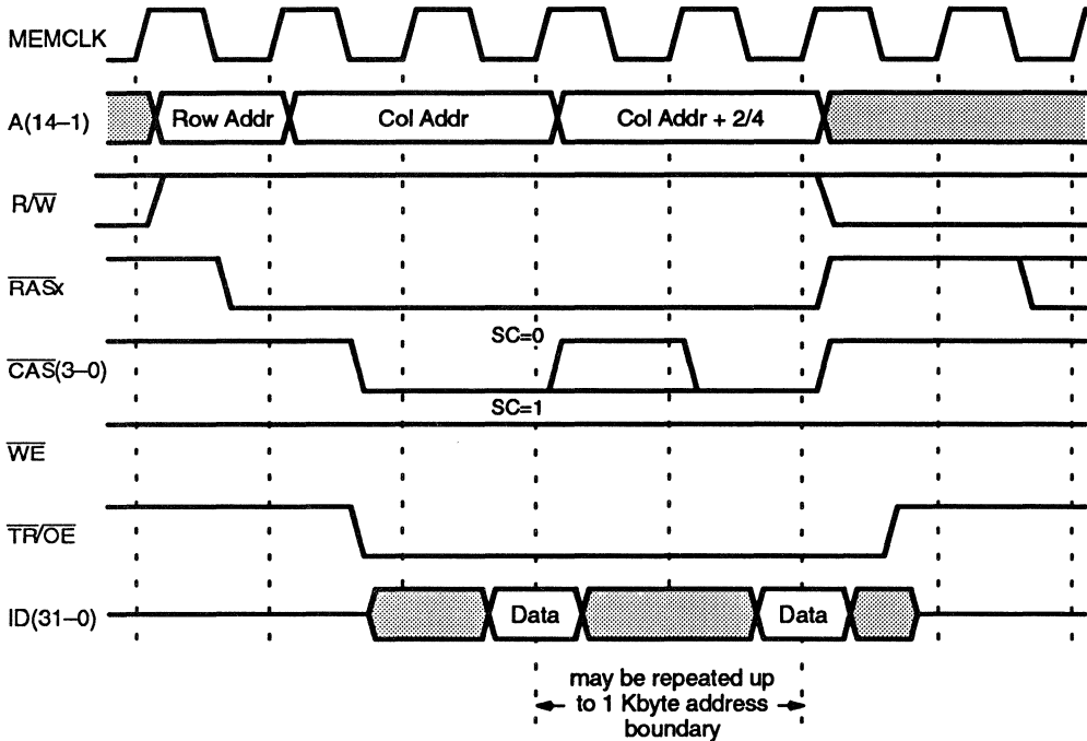
Figure 9-7 DRAM Page-Mode Read Cycle
