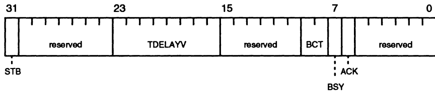
Figure 13-2 Parallel Port Status Register
