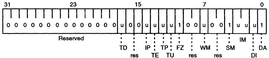
Figure 17-4 Processor Status While in Load Test Instruction Mode
