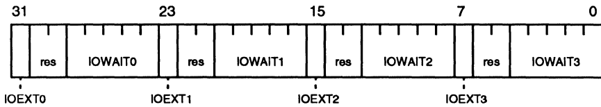
Figure 10-1 PIA Control Register 0 (PICT0, Address 80000020)
