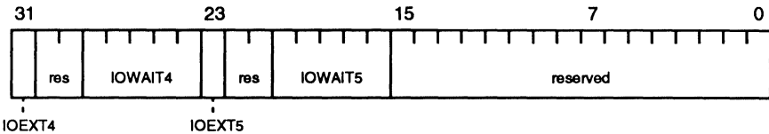
Figure 10-2 PIA Control Register 1 (PICT1, Address 80000024)
