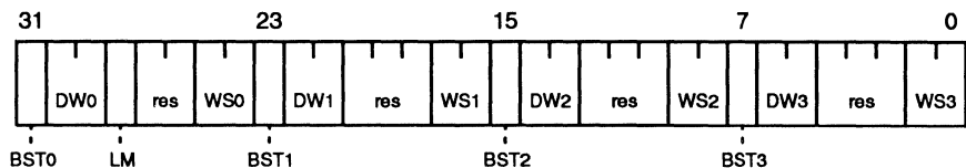
Figure 8-1 ROM Control Register
