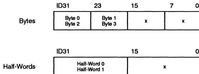
Figure 9-4 Location of Bytes and Half-Words on a 16-Bit Bus
