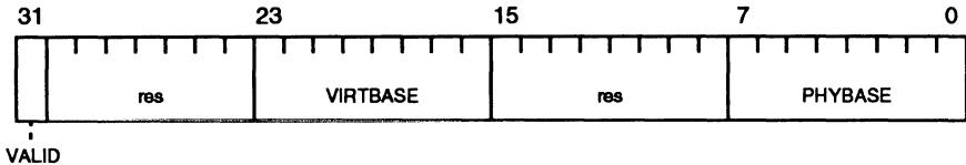
Figure 9-3 DRAM Mapping Register 0
