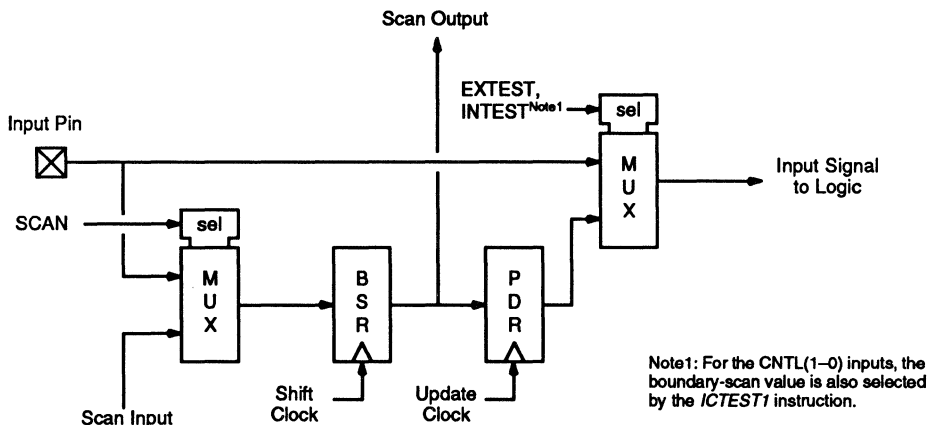
Figure 17-2 Input Boundary-Scan Cell
