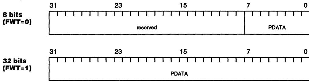
Figure 13-3 Parallel Port Data Register
