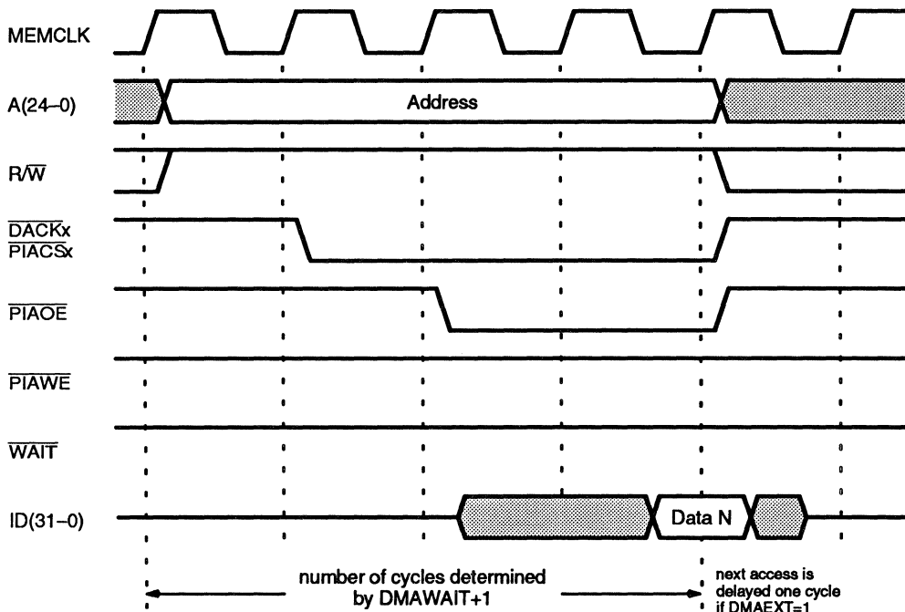
Figure 11-6 DMA Read Cycle
