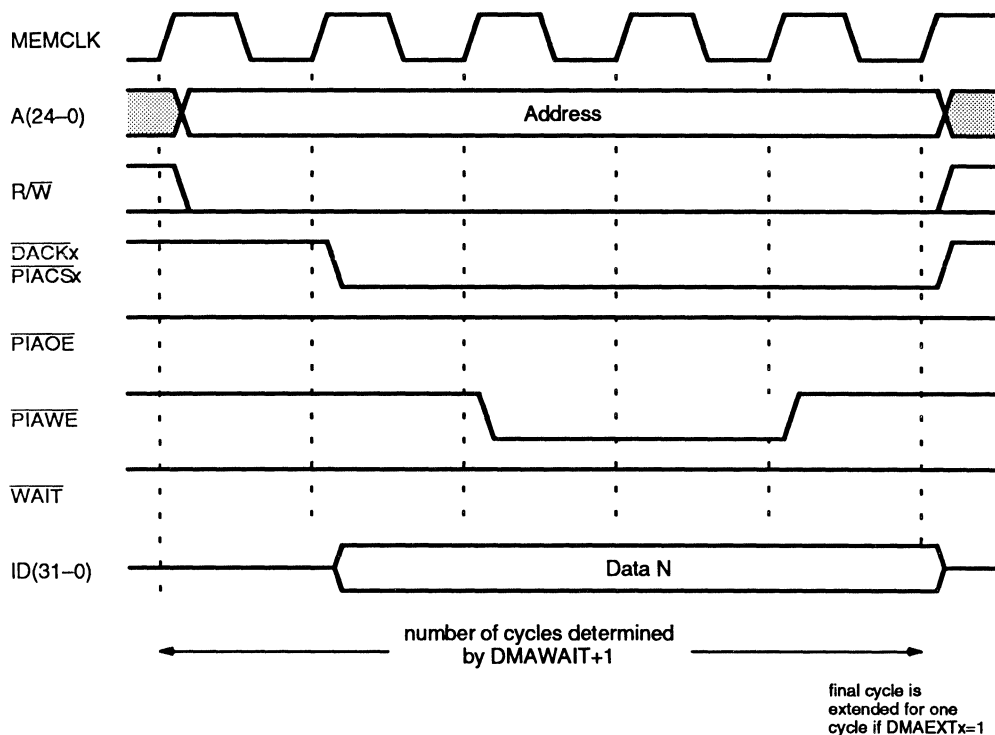
Figure 11-7 DMA Write Cycle
