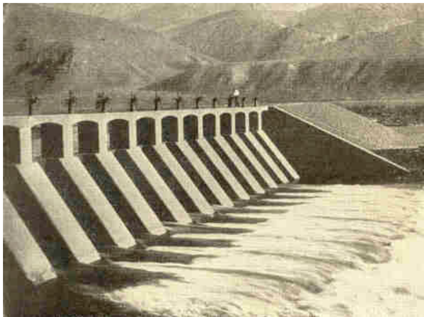
Truckee-Carson reclamation project. Diversion dam and gates at heading of main canal.
