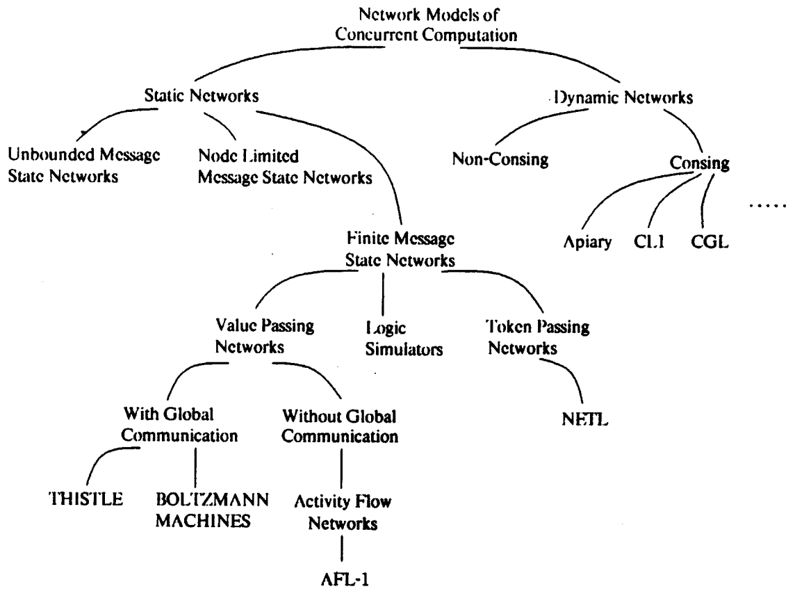
Figure 2.1: A Taxonomy of Concurrent Network Models.
