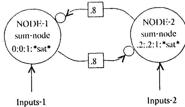
Figure 7.4: Implementation of a Two Member Type 3 ME-Group.
