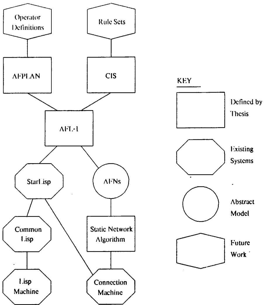
Figure 1.7: Levels of Systems Discussed in this Thesis.
