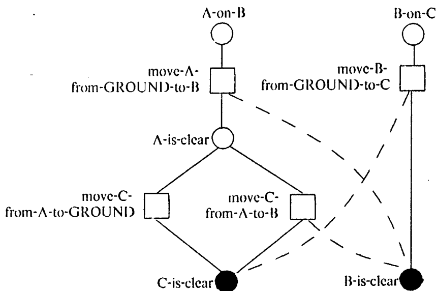
Figure 6.3: The Part of the AFN Activated by the Anomalous Situation. Dark circles show the active states, and dashed lines show preconditions that get deleted (deactivated) if the operator they are linked to is applied.
