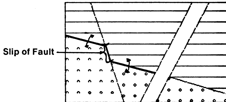
Fig. 19. Measuring the Slip of a Fault
