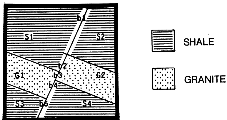
Fig. 16. Relations Between Diagram and Geologic Features
