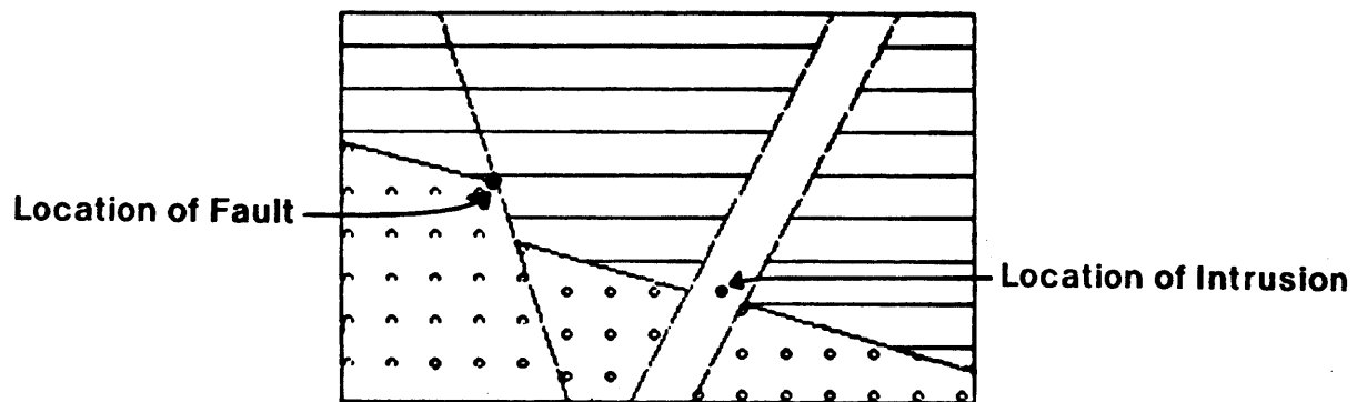
Fig. 20. Measuring the Location of a Boundary
