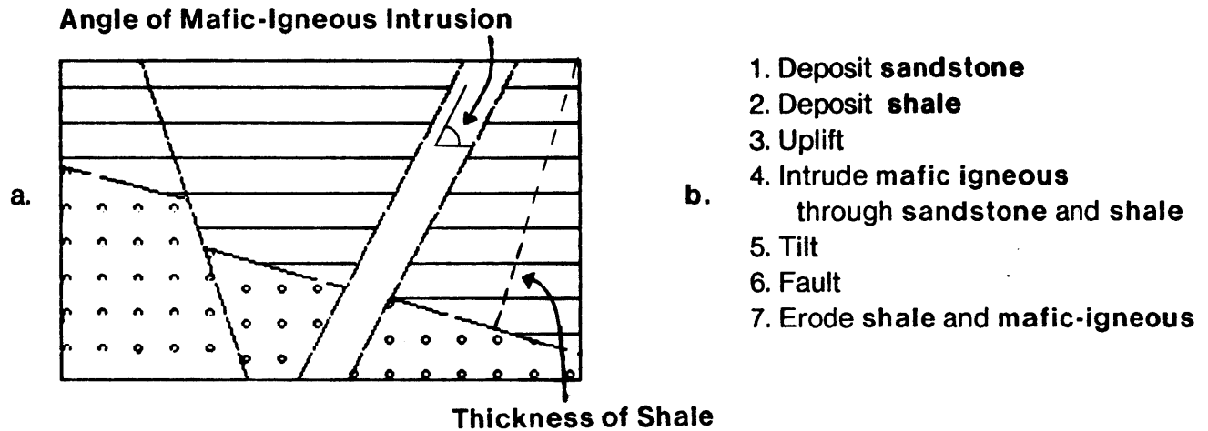
Fig. 6. Measuring from the Diagram
