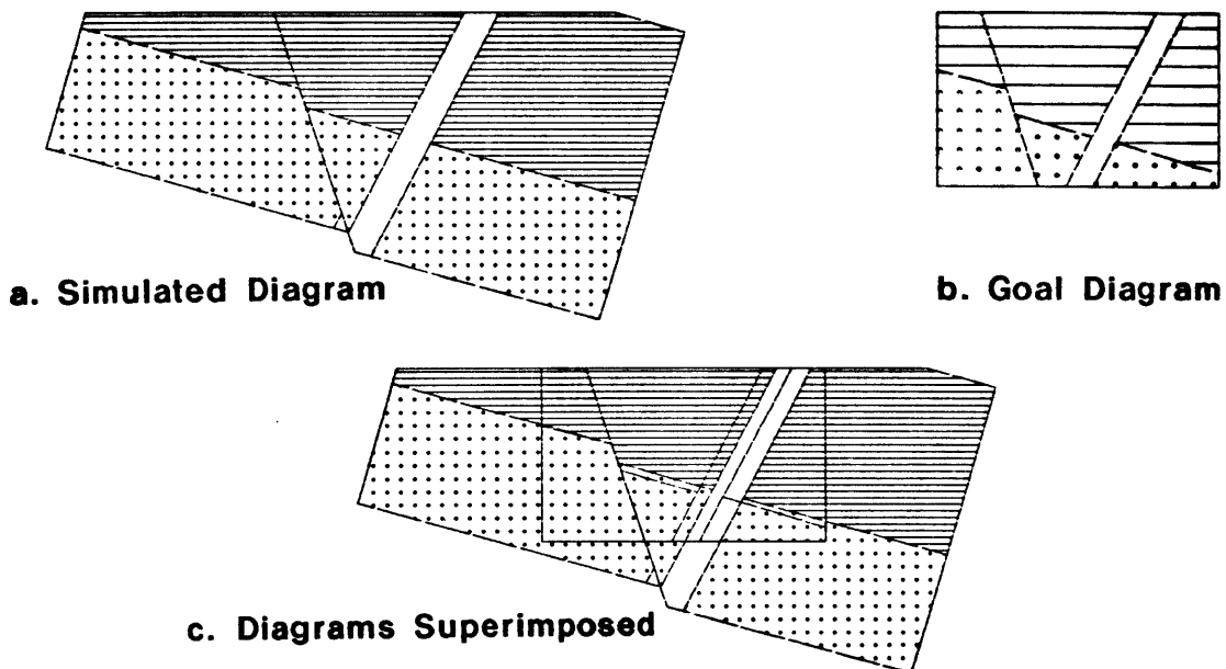
Fig. 28. Quantitative Simulation Using Incomplete Process Description
