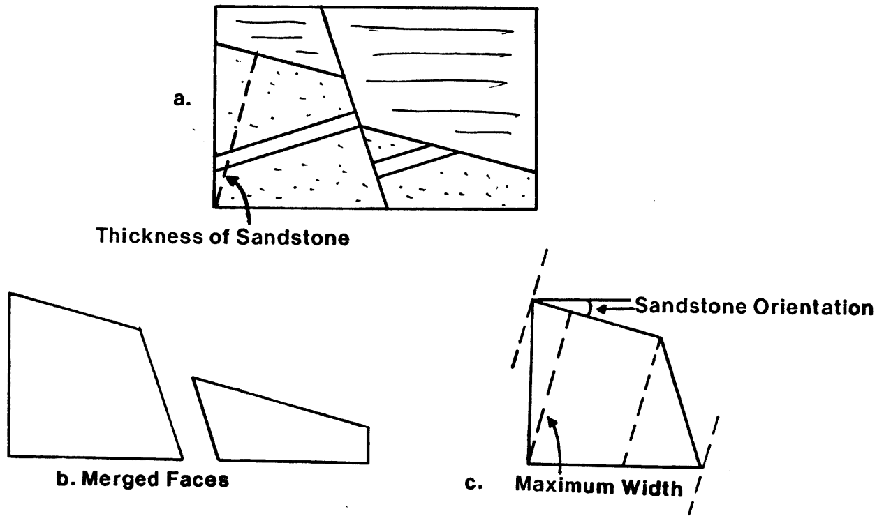
Fig. 21. Measuring the Thickness of a Rock-Unit
