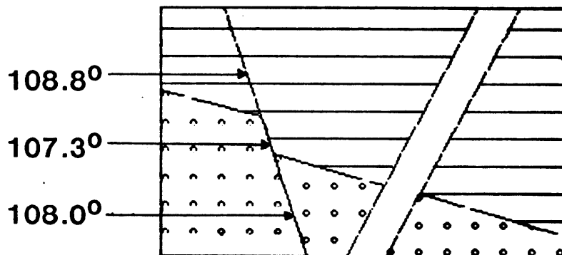
Fig. 10. Fault Drawn in the Goal Diagram is not Straight
