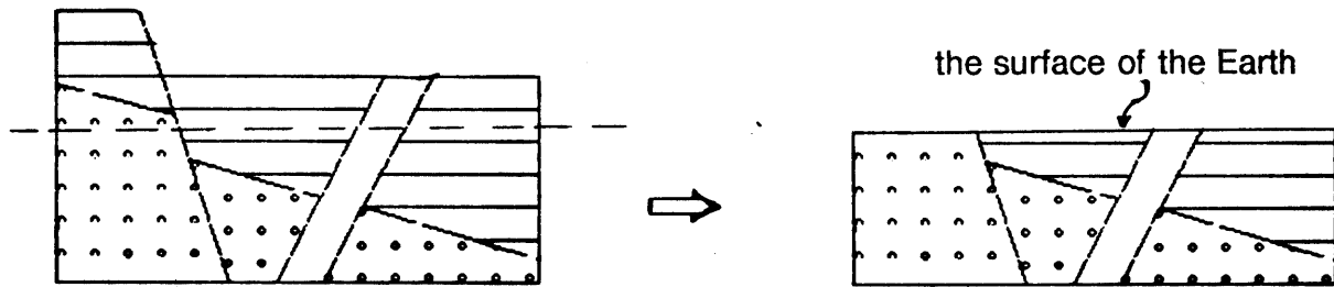
Fig. 9. Quantitative Simulation of Erosion
