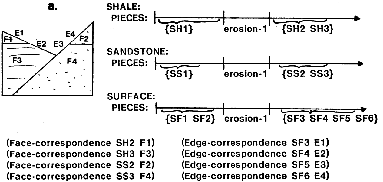
Fig. 27. Maintaining the Piece Structure When Manipulating Diagrams
