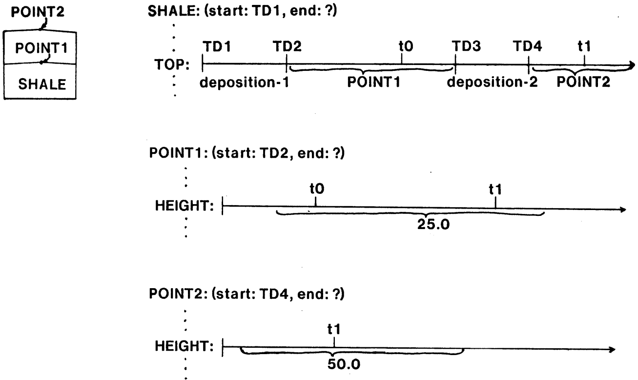
Fig. 12. History Representation after Deposition of More Shale
