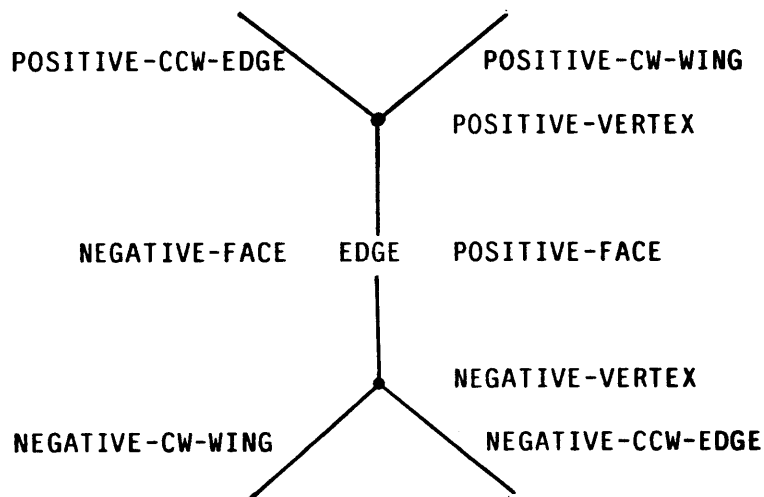
Fig. 15. The Wing-Edge Representation of an Edge
