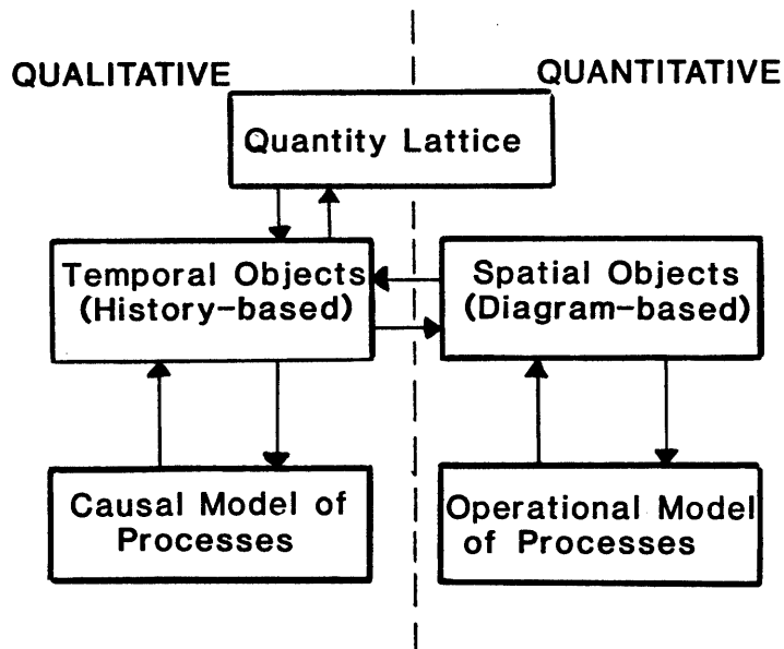
Fig. 2. Representations for Doing Imagining
