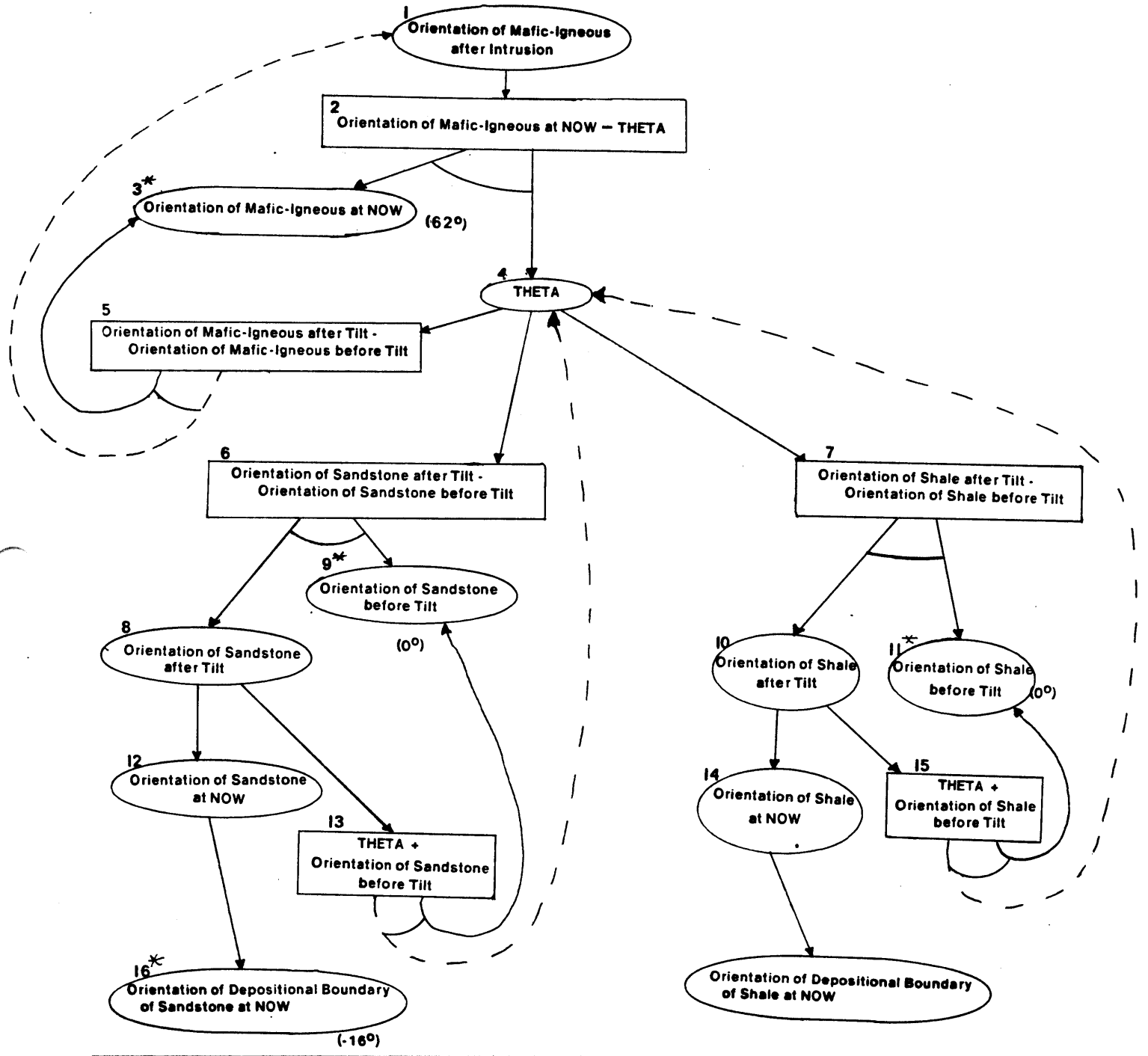
Fig. 8. Partial AND-OR Graph for Parameter Determination
