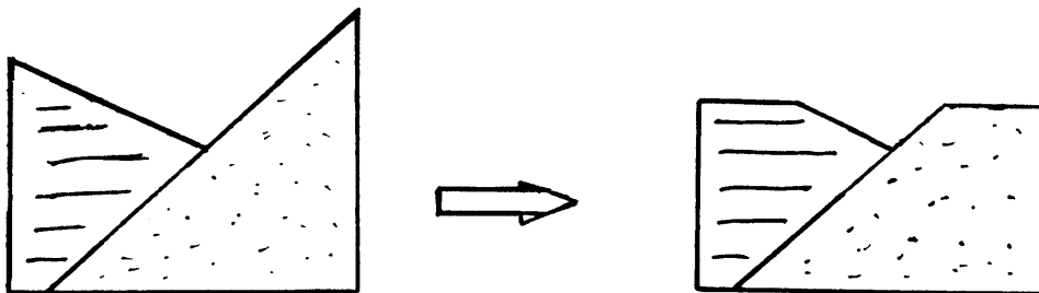
Fig. 25. Erosion Above Bottom of Earth's Surface
