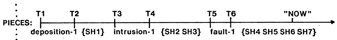
Fig. 17. Representation of the Pieces of Shale
