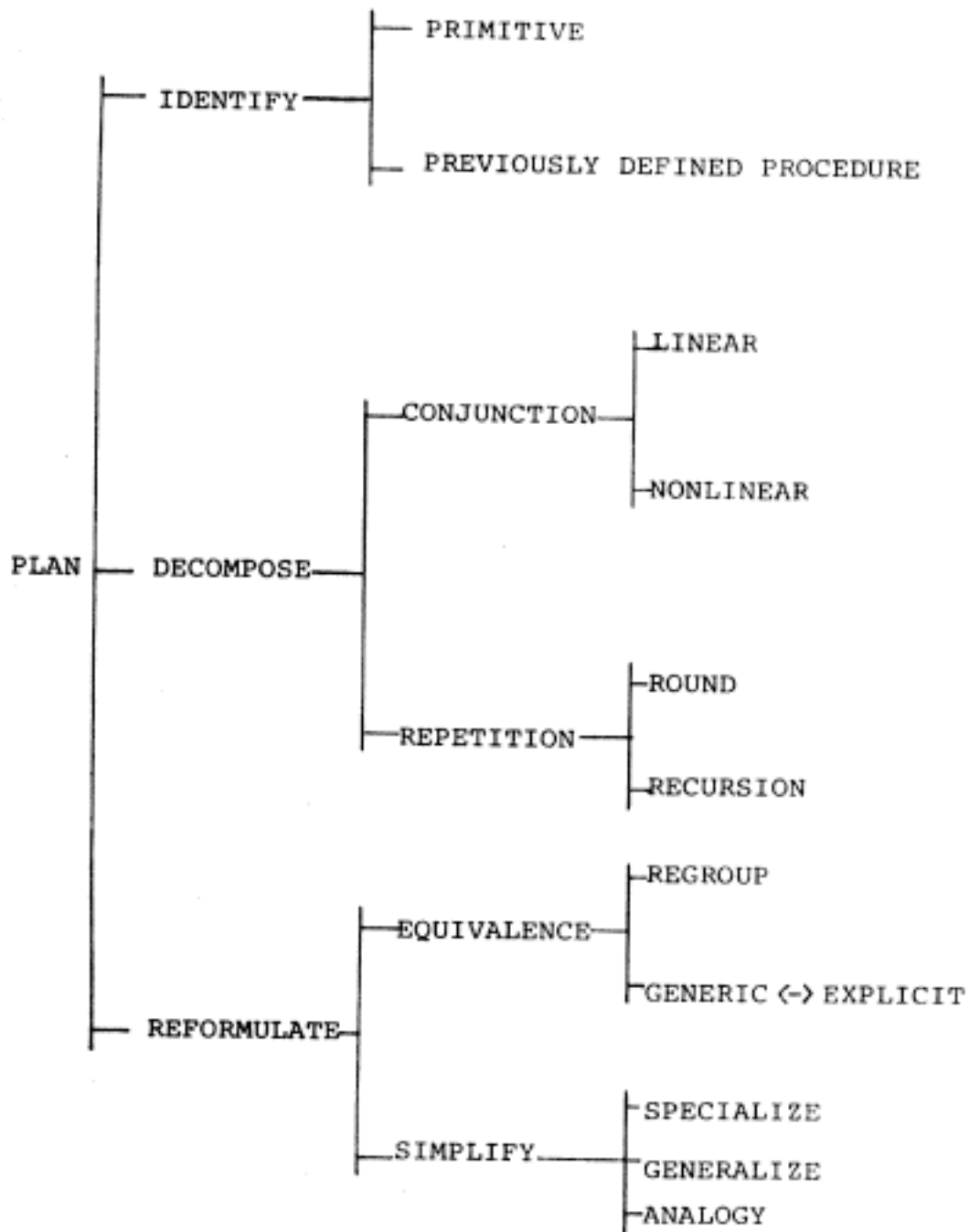
FIGURE 1 TAXONOMY OF PLANNING CONCEPTS
