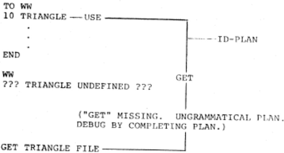
FIGURE 4 - SEMANTICALLY INCORRECT PLAN AN OPTIONAL CONJUNCT IS MISSING
