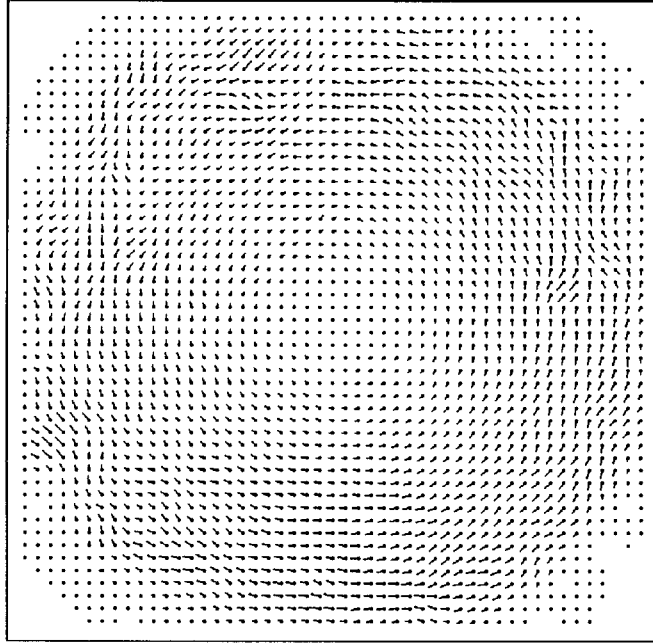
Figure 6: The optical flow field (rotating circle) generated by the local constraint algorithm, followed by Gaussian smoothing (on each component), with \sigma = 3 .
