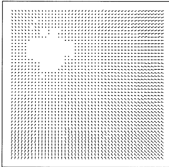
Figure 12: Optical flow (looming image) produced by the matching algorithm using a displacement range of \pm 8 pixels.
