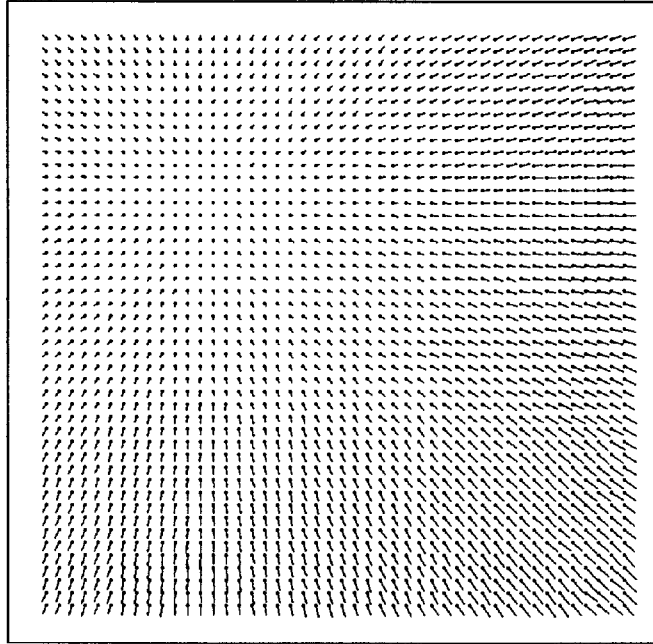
Figure 9: The optical flow (looming image) produced after 400 iterations by the Horn-Schunck algorithm, as in [Hor85], with \lambda = 1 .
