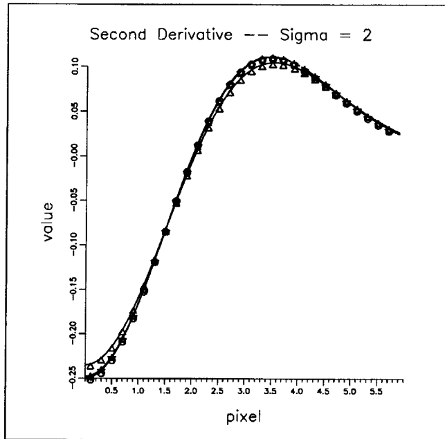
Figure 16: The second derivative of the Gaussian function ( \sigma = 2 ): derivative of the Gaussian (open circle); central difference (triangle); five-point formula (star).
