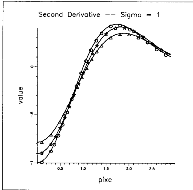
Figure 15: The second derivative of the Gaussian function ( \sigma = 1 ): derivative of the Gaussian (open circle); central difference (triangle); five-point formula (star).
