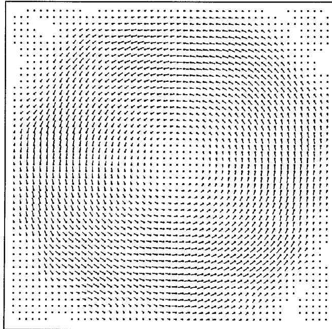
Figure 7: The optical flow field (rotating circle) generated by the gradient constancy algorithm, followed by Gaussian smoothing (on each component), with \sigma = 3 .
