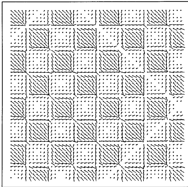
Figure 3: Normal flow obtained by solving Eq. 2 at the third of five frames. Image brightness derivatives have been computed by using five-point approximation of derivatives derived by means of Taylor's expansion.
