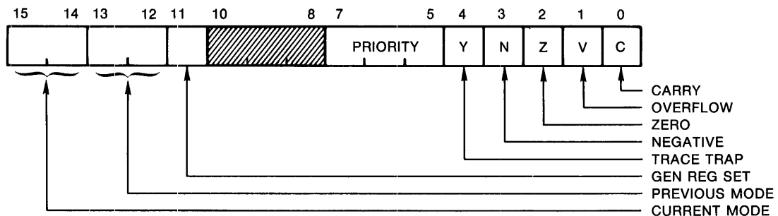
Figure B-1 Format of the Processor Status Word
